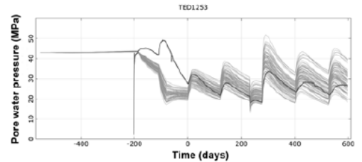
Figure 7: pore water pressure at the measurement point 1253 with a scattering range of the simulation model.
