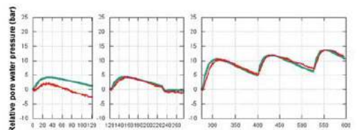
Figure 8b: Comparison of simulation vs. measurement at point 1252 after the parameter identification: Relative pore water pressure of the three heating periods.
