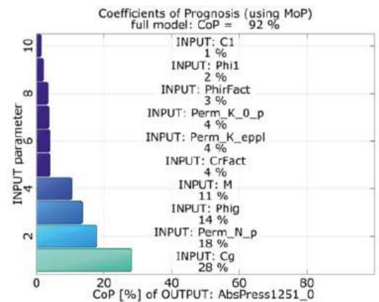
Figure 4: CoP relative pore pressure at time t = 0 , the measuring point in 1251.
