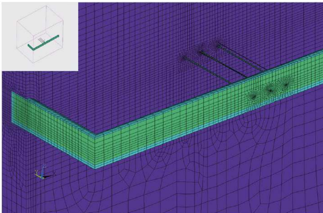
Figure 1: FE-mesh of structure, section.
