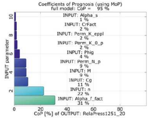
Figure 5: CoP relative pore pressure at time t = 20 days, measurement point 1251.
