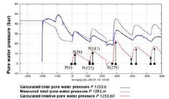
Figure 3: Relative pore water pressures for parameter identification.
